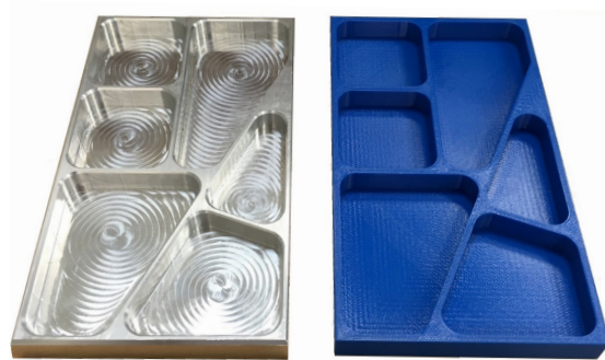
Figure 1: CNC (aluminum) on the left, 3D printed (plastic), right.
