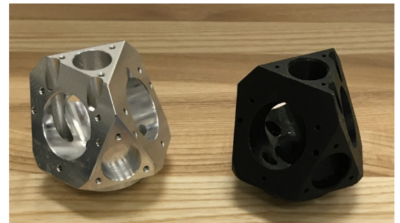
Figure 2: CNC (aluminum) on the left, 3D printed (plastic), right.
